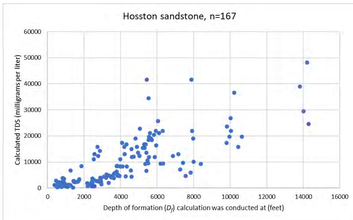
Figure 11-22 Depth of formation ( D_f ) in feet and the calculated total dissolved solids (TDS) in milligrams per liter for the Hosston sandstone.
