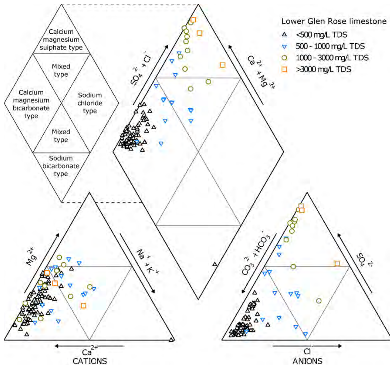
Figure 10-9 Piper plots of the Lower Glen Rose limestone, with data points symbolized by water quality (<500, 500-1,000, 1,000-3,000, and >3,000 milligrams per liter total dissolved solids). Number of samples is 104.
