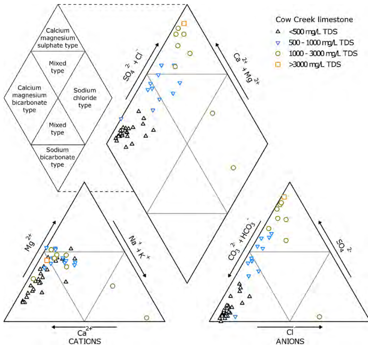
Figure 10-13 Piper plots of the Cow Creek limestone, with data points symbolized by water quality ( <500 , 500-1,000, 1,000-3,000, and >3,000 milligrams per liter total dissolved solids). Number of samples is 46.
