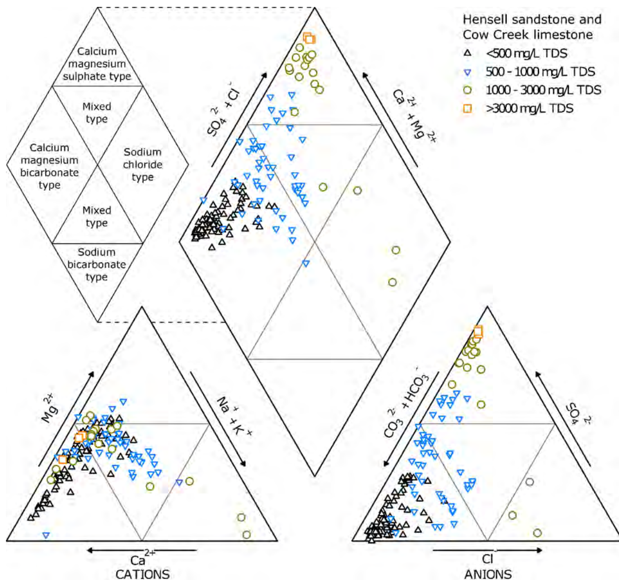
Figure 10-11 Piper plots of the Hensell sandstone and Cow Creek limestone, with data points symbolized by water quality (<500, 500-1,000, 1,000-3,000, and >3,000 milligrams per liter total dissolved solids). Number of samples is 150.
