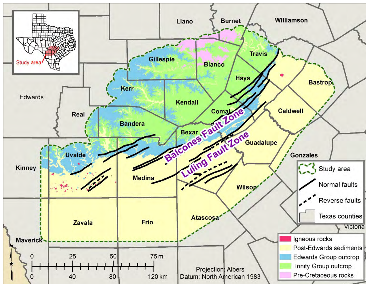
Figure 1-2 Hill Country Trinity Group simplified geologic setting.
