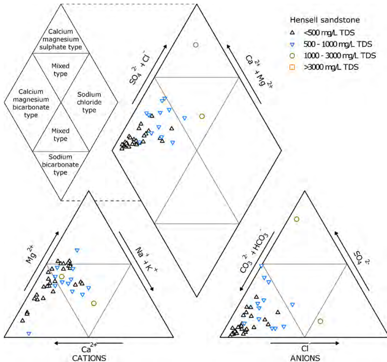
Figure 10-12 Piper plots of the Hensell sandstone, with data points symbolized by water quality (<500, 500-1,000, 1,000-3,000, and >3,000 milligrams per liter total dissolved solids). Number of samples is 43.
