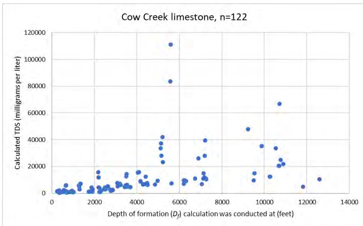
Figure 11-20 Depth of formation ( D_f ) in feet and the calculated total dissolved solids (TDS) in milligrams per liter for the Cow Creek limestone.
