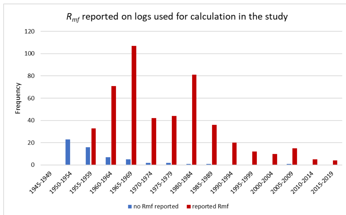
Figure 11-4 Distribution of logs used to calculate estimated groundwater salinity with and without a header reported R_{mf} value by five-year interval from 1945-2019.
