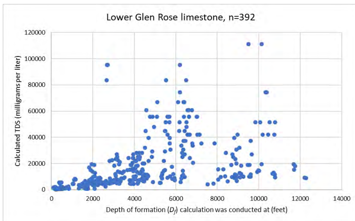
Figure 11-18 Depth of formation ( D_f ) in feet and the calculated total dissolved solids (TDS) in milligrams per liter for the Lower Glen Rose limestone.
