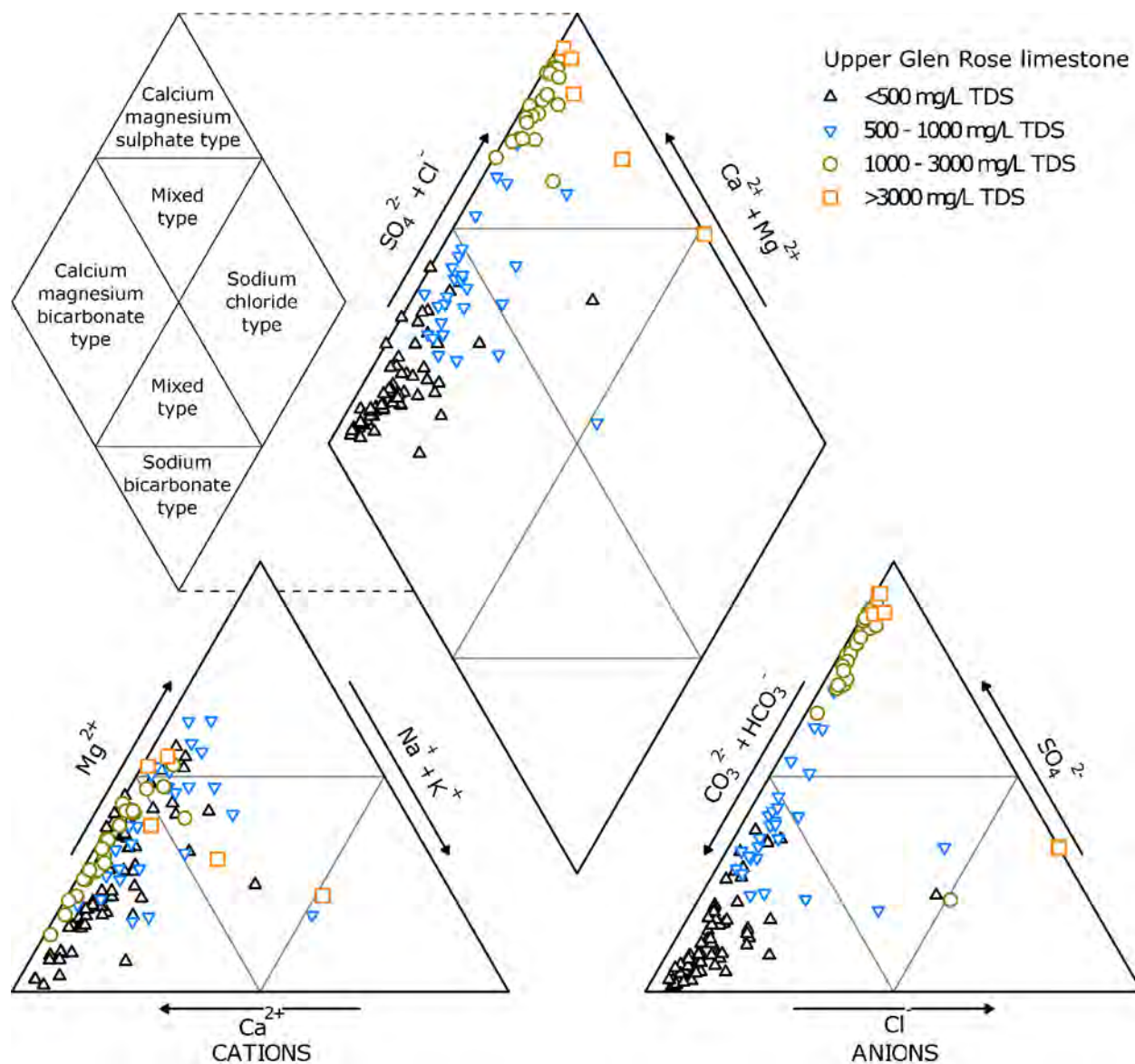
Figure 10-8 Piper plots of the Upper Glen Rose limestone, with data points symbolized by water quality (<500, 500-1,000, 1,000-3,000, and >3,000 milligrams per liter total dissolved solids). Number of samples is 127.
