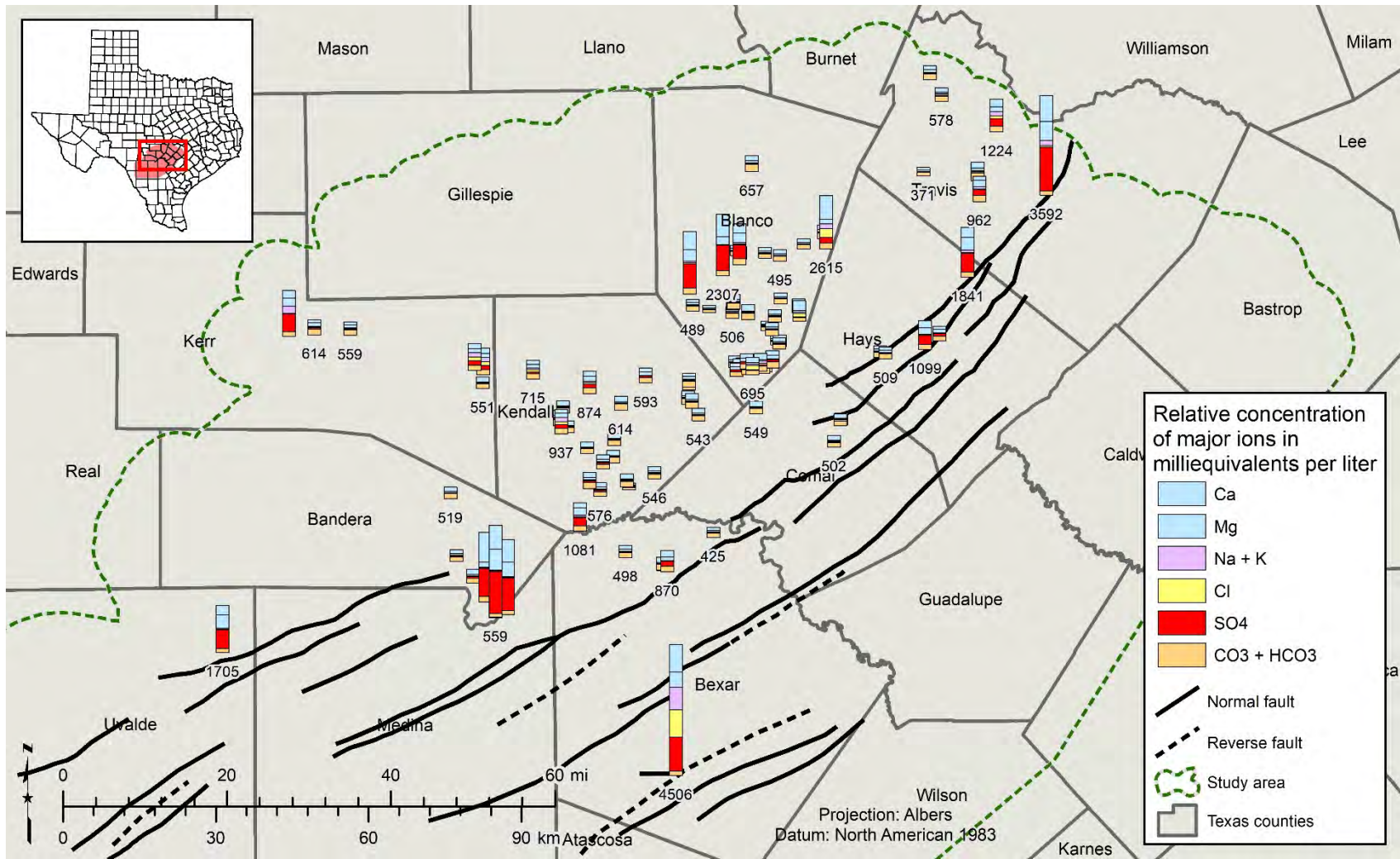
Figure 10-19 Map of water quality samples for the Lower Glen Rose limestone showing the relative proportion of the major ions in milliequivalents per liter as a stacked bar chart for each well. Milligrams per liter total dissolved solids are labeled beneath some of the wells for reference. Number of well locations is 104. (Ca = calcium, Mg = magnesium, Na = sodium, K = potassium, Cl = chloride, SO 4 = sulfate, CO 3 = carbonate, HCO 4 = bicarbonate)
