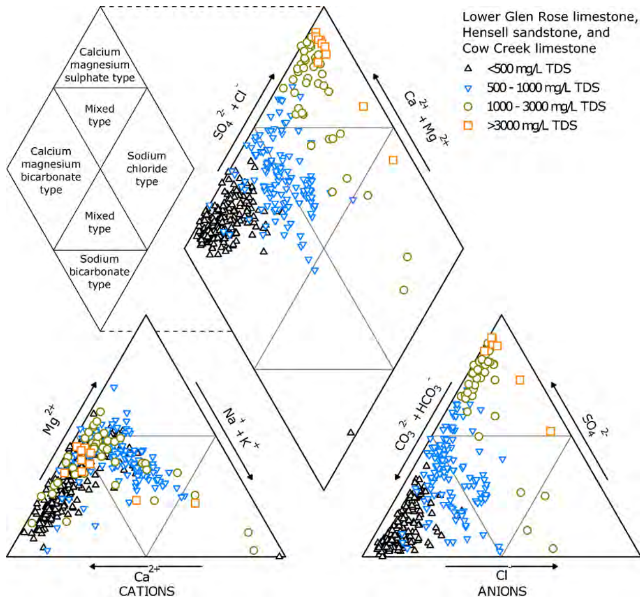
Figure 10-10 Piper plots of the Lower Glen Rose limestone, Hensell sandstone, and Cow Creek limestone, with data points symbolized by water quality (<500, 500-1,000, 1,000-3,000, and >3,000 milligrams per liter total dissolved solids). Number of samples is 484.
