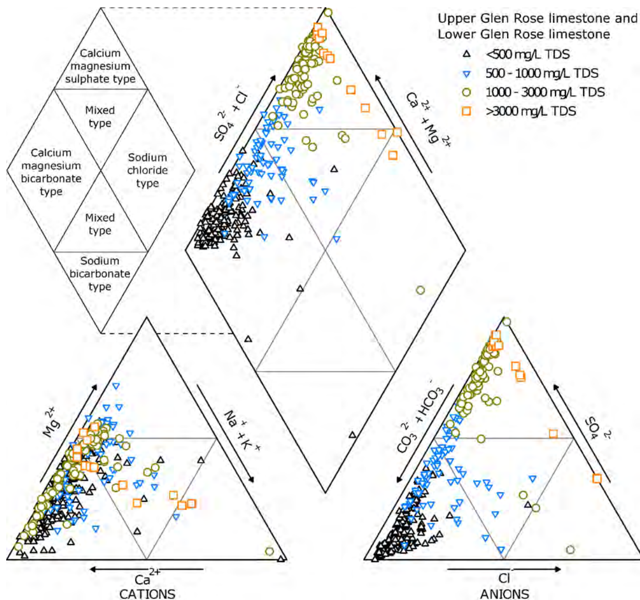
Figure 10-7 Piper plots of the Upper Glen Rose limestone and Lower Glen Rose limestone, with data points symbolized by water quality (<500, 500-1,000, 1,000-3,000, and >3,000 milligrams per liter total dissolved solids). Number of samples is 393.
