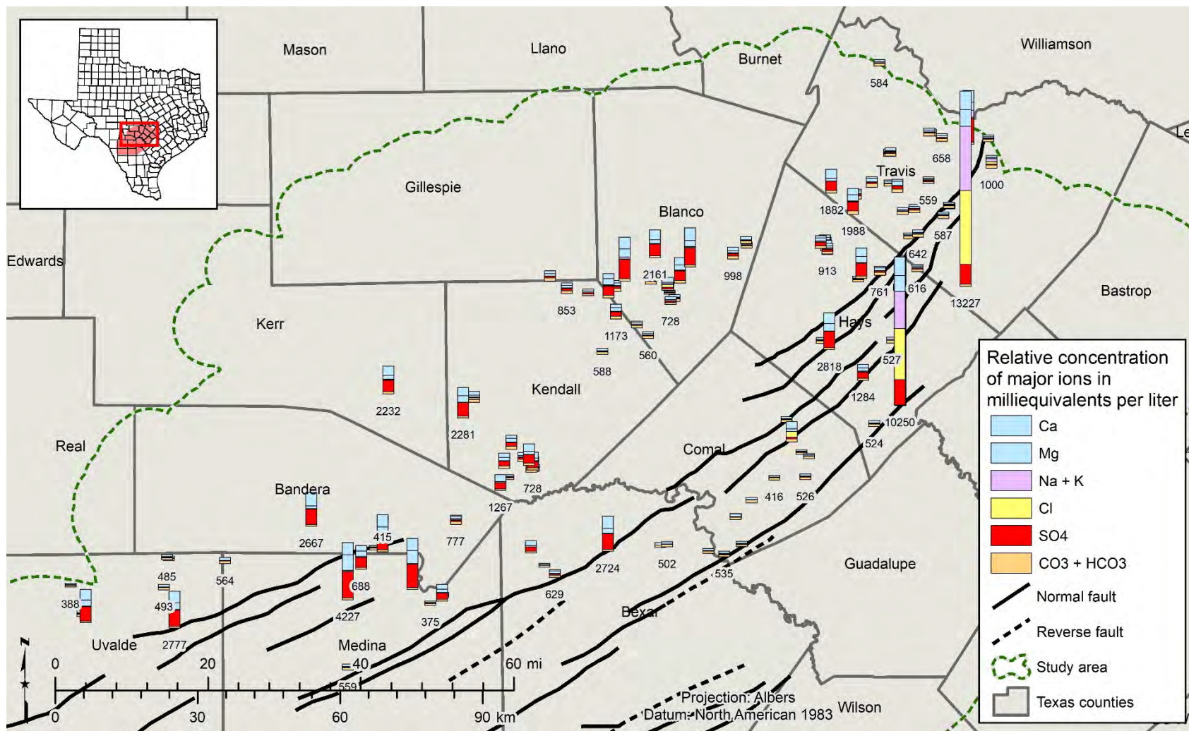
Figure 10-18 Map of water quality samples for the Upper Glen Rose limestone showing the relative proportion of the major ions in milliequivalents per liter as a stacked bar chart for each well. Milligrams per liter total dissolved solids are labeled beneath some of the wells for reference. Number of well locations is 128. (Ca = calcium, Mg = magnesium, Na = sodium, K = potassium, Cl = chloride, SO 4 = sulfate, CO 3 = carbonate, HCO 4 = bicarbonate)
